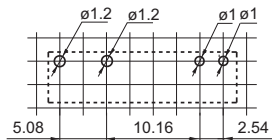
HF49FD/□□□ -1H□1(XXX)
