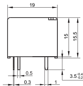
Outline Dimensions
