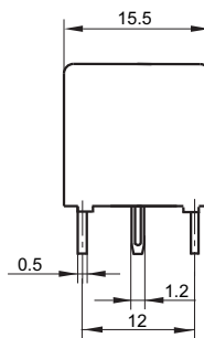
Outline Dimensions
