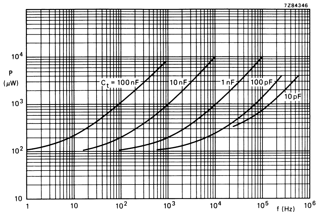
Fig.10 Power consumption as a function of the output frequency at O or \overline{O} ; V_{DD} = 5 V; astable mode.
