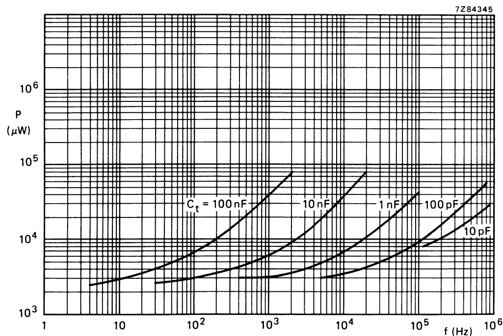
Fig.11 Power consumption as a function of the output frequency at O or \overline{O} ; V_{DD} = 10 V; astable mode.
