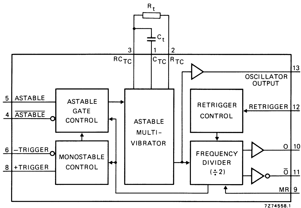
Fig.1 Functional diagram.
