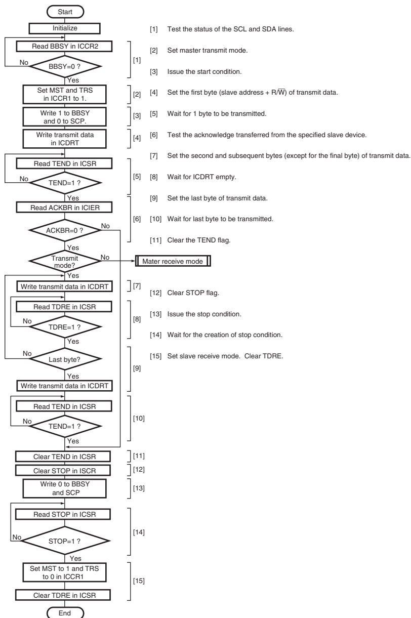
Figure 15.17 Sample Flowchart for Master Transmit Mode
