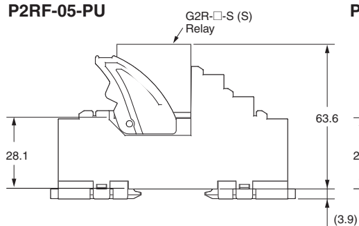
P2RF-□
