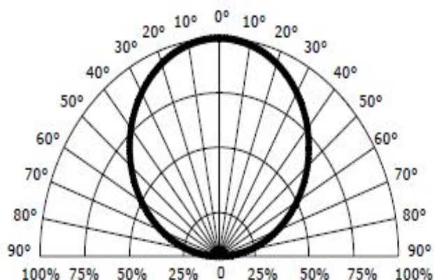
Fig. 6 Relative Luminous Flux vs Radiation Angle
