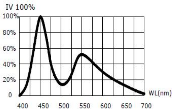
Fig. 4 Relative Luminous Flux vs Wavelength
