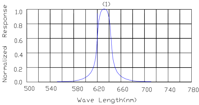
Spectral Radiance
