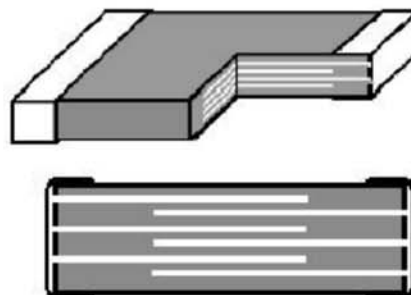
Section of the chip
