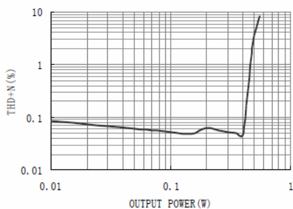
THD+N vs OutputPower VDD=3.3V, RL=8Ω, and f=1KHz
