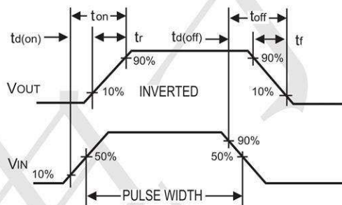
Figure 18. Switching Waveforms
