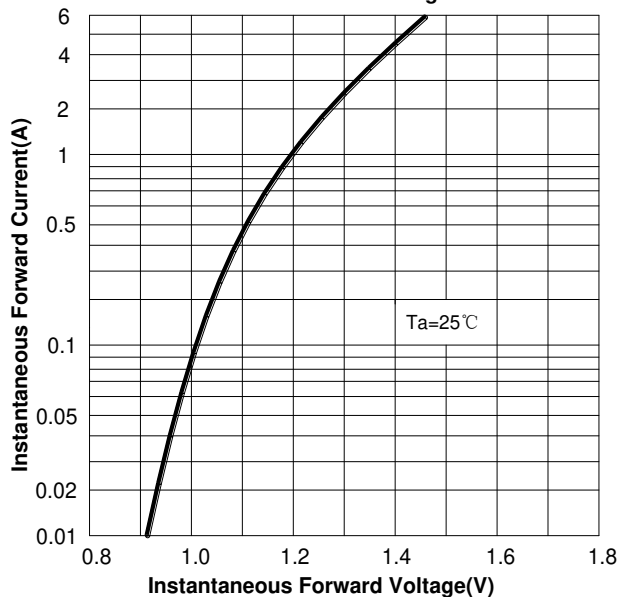
FIG3: Forward Voltage
