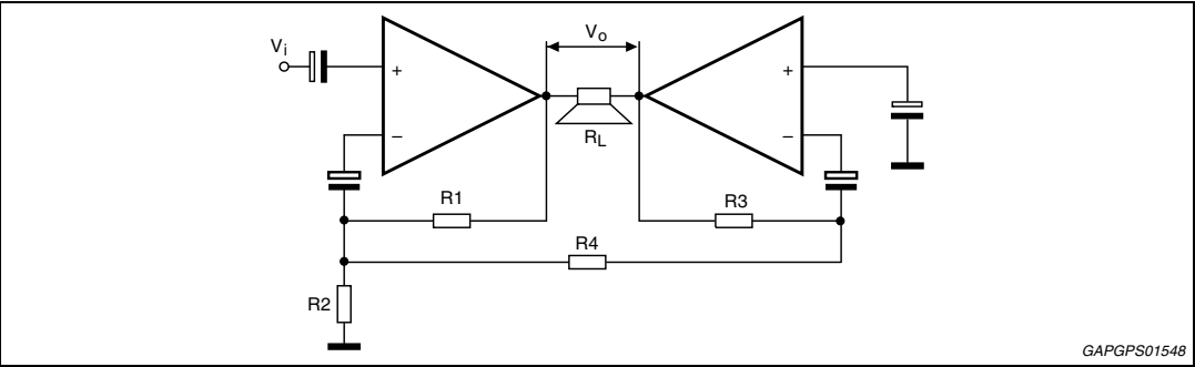
Figure 8. Bridge configuration
