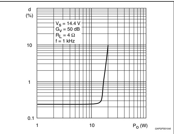
Figure 6. Distortion vs. output power ( R_L = 4 \text{ } \Omega )
