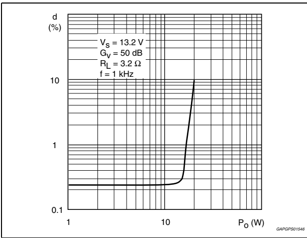
Figure 7. Distortion vs. output power ( R_L = 3.2 \text{ } \Omega )
