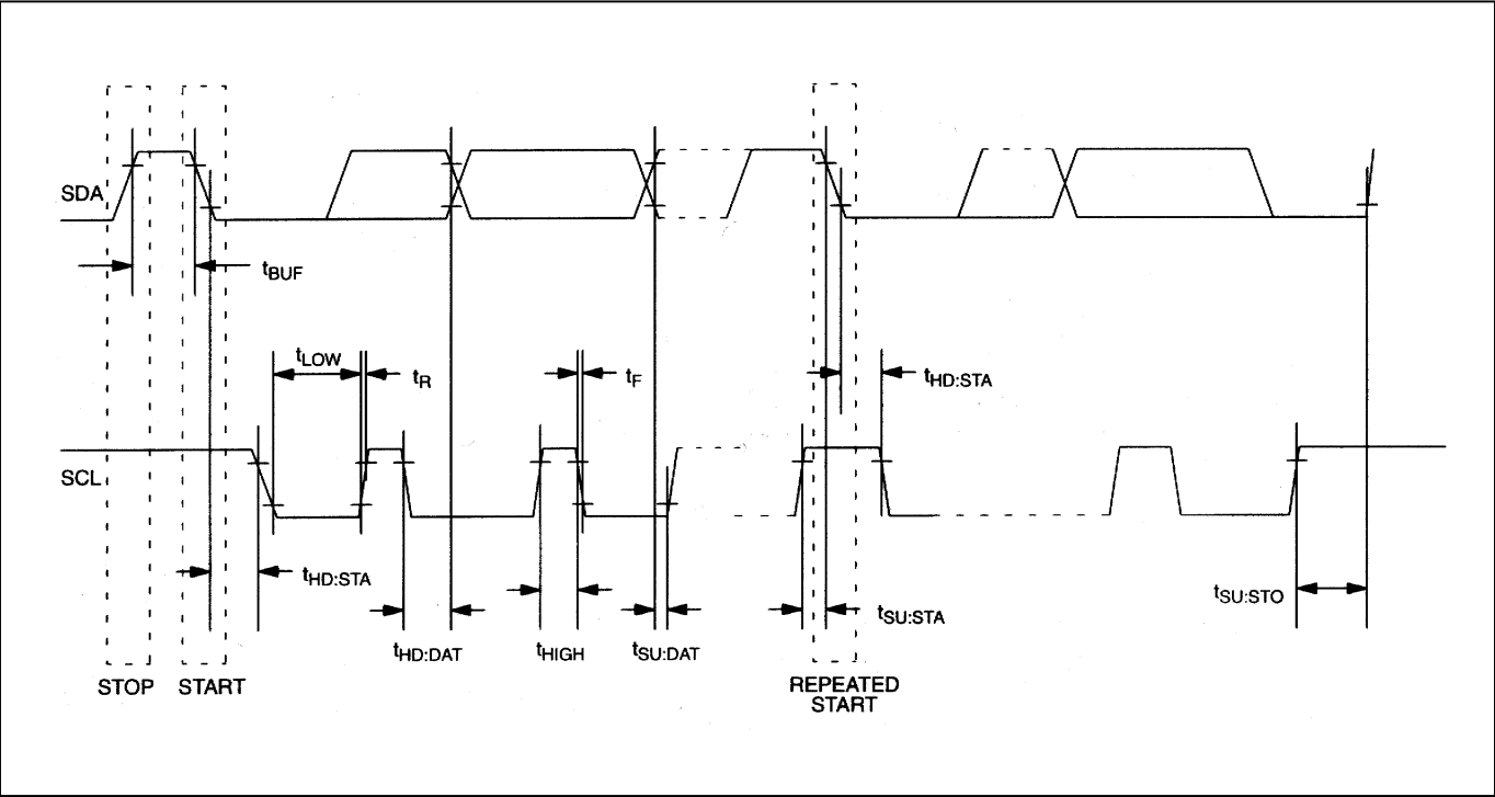
Figure 2. Timing Diagram
