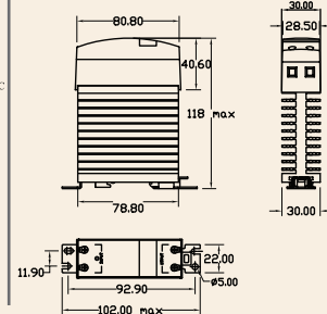
Mechanical Drawing
