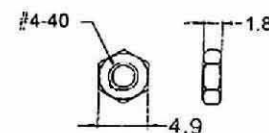
NUT: STEEL IN NICKEL PLATED (2 pcs)
