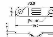
CABLE CLAMP: STEEL IN NICKEL PLATED (2 pcs)
