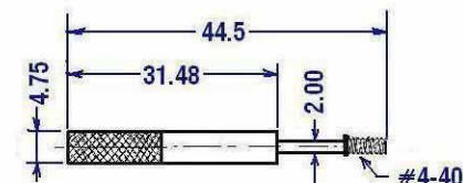
LONG SCREW: STEEL IN NICKEL PLATED (2 pcs)
