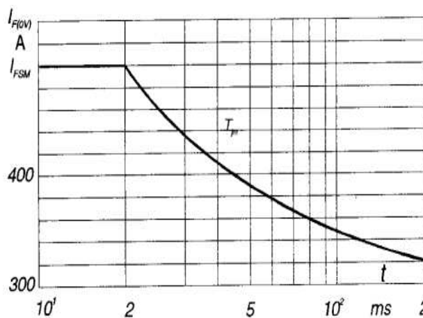
Maximum overload characteristic.
