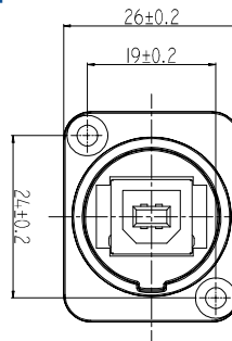
Panel cut out (Rear side)
