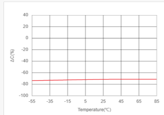
Bias TCC Characteristics LCR meter, 0.12kHz, 0.5Vrms, 5Vdc
