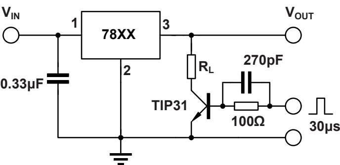
Figure 9-6. Load Regulation
