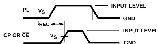
FIGURE 8. SERIAL-SHIFT MODE
