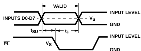
FIGURE 6. PARALLEL-LOAD MODE
