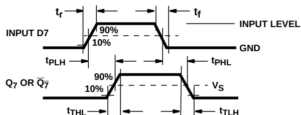
FIGURE 5. PARALLEL-LOAD MODE
