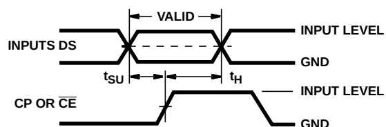
FIGURE 7. SERIAL-SHIFT MODE
