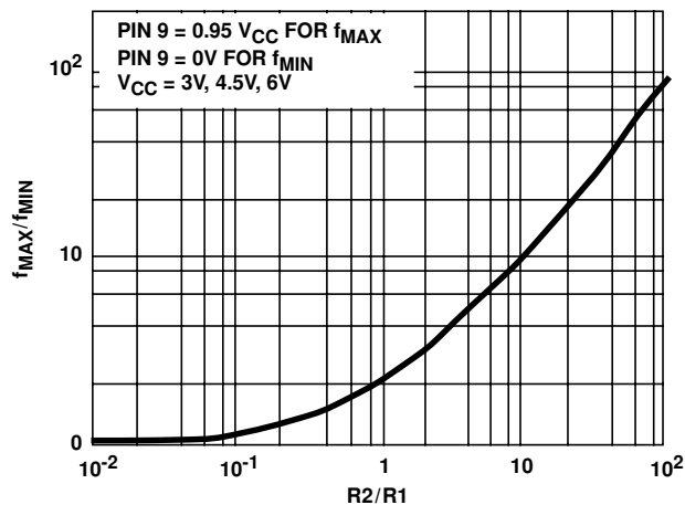
FIGURE 31. HC4046A f_{MAX}/f_{MIN} vs R2/R1 ( V_{CC} = 3V, 4.5V, 6V )
