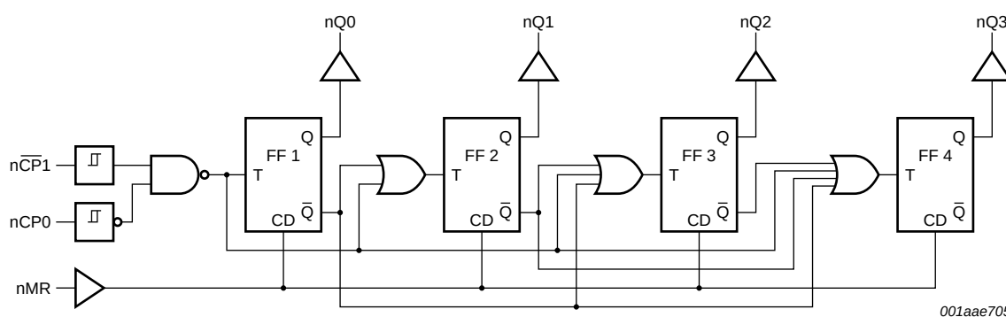
Fig 3. Logic diagram for one counter
