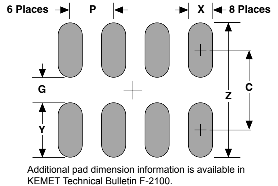
1632 CERAMIC ARRAY LAND PATTERN LAYOUT
