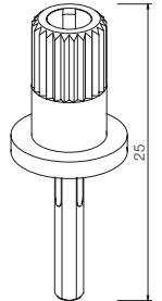
9048 For 2 potentiometers
