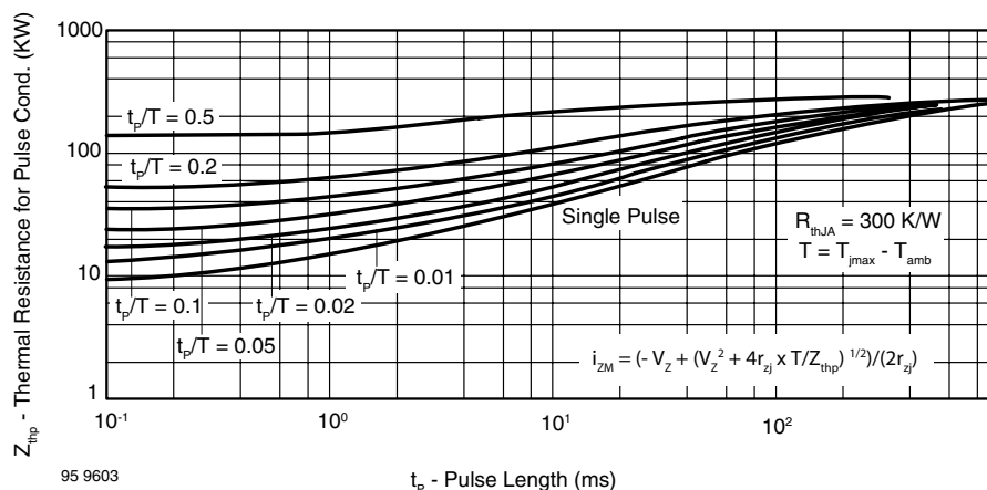
Figure 13. Thermal Response
