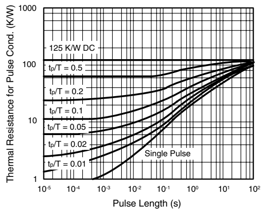
Figure 8. Thermal Response
