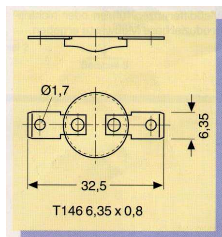
Terminals T 146
