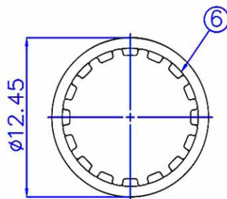
LOCK WASHER
