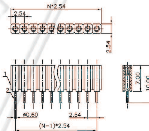
SINGLE ROW
