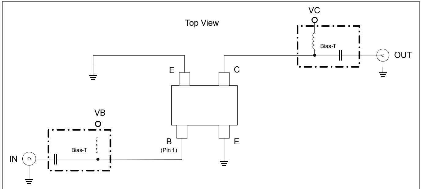
Figure 4 Testing circuit
