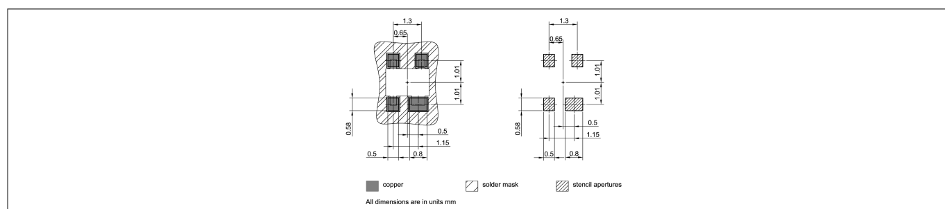
Figure 21 Foot print
