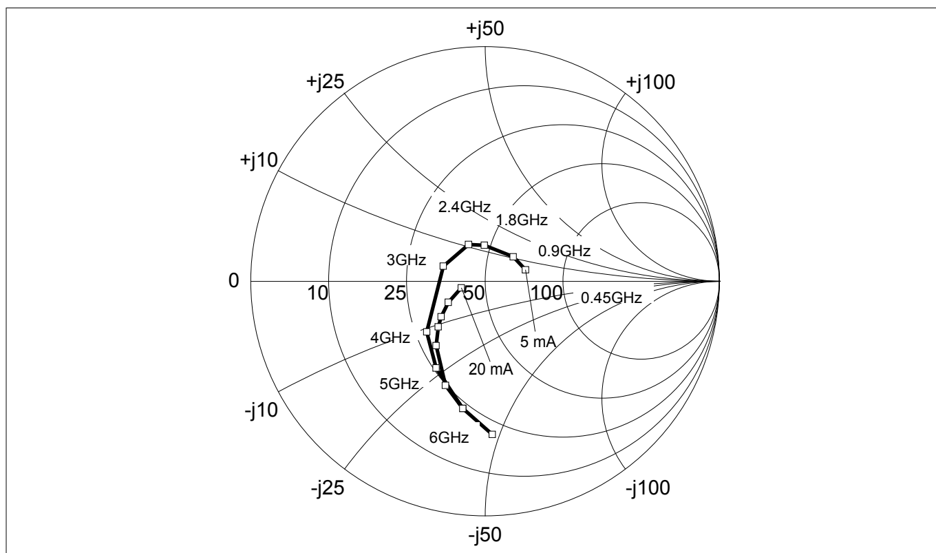
Figure 16 Source impedance for minimum noise figure Z_{S,\text{opt}} = f(f) , V_{CE} = 2 \text{ V} , I_C = 5 / 20 \text{ mA}
