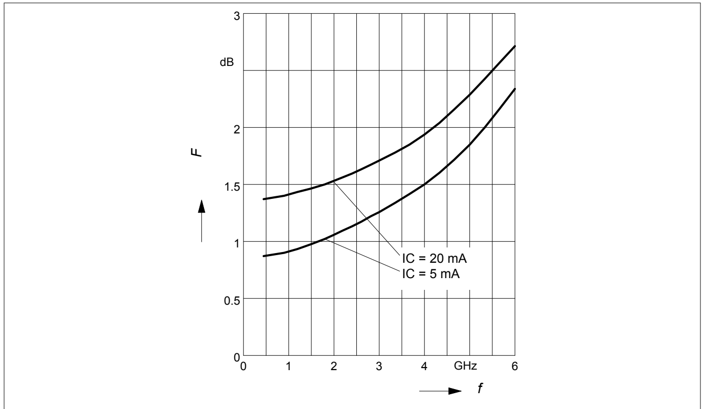
Figure 17 Noise figure NF_{\min} = f(f) , V_{CE} = 2 \text{ V} , Z_S = Z_{S,\text{opt}} , I_C = 5 / 20 \text{ mA}
