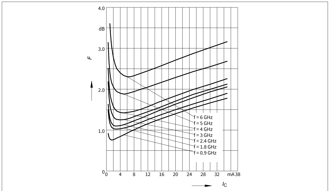
Figure 18 Noise figure NF_{\min} = f(I_C) , V_{CE} = 2 \text{ V} , Z_S = Z_{S,\text{opt}} , f = \text{parameter in GHz}
