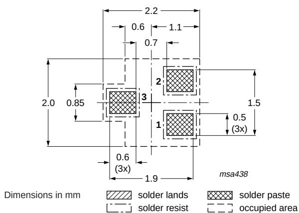
Fig 17. Reflow soldering footprint BAV70T (SOT416/SC-75)
