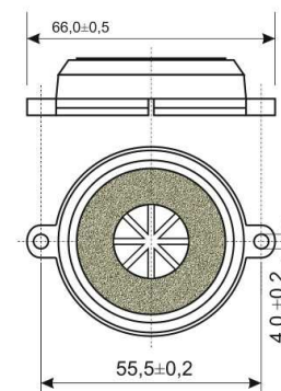
HOUSING 3
