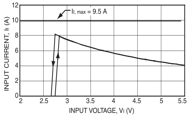
Figure 1. Typical Input Characteristic at 10A Output Current.
