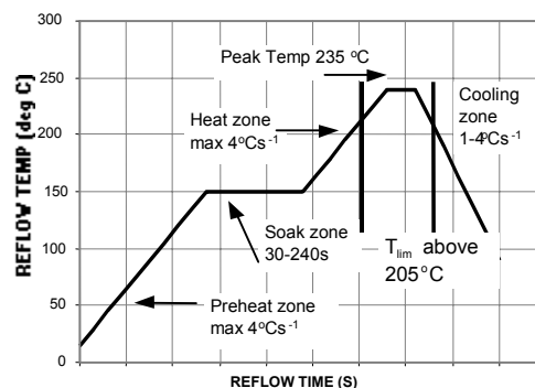
Figure 29. Reflow Profile.
