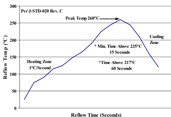
Figure 31. Recommended linear reflow profile using Sn/Ag/Cu solder.
