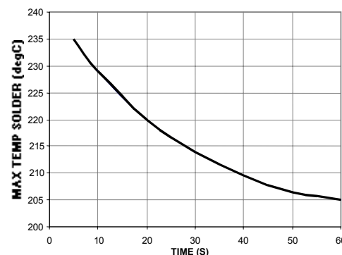
Figure 29. Reflow Profile.
