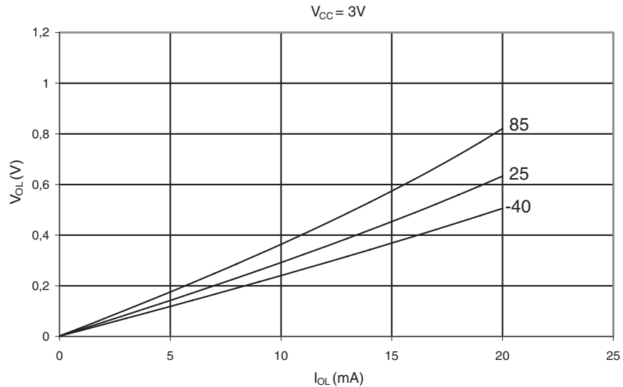
Figure 24-19. I/O Pin Output Voltage vs. Sink Current ( V_{CC} = 3V )
