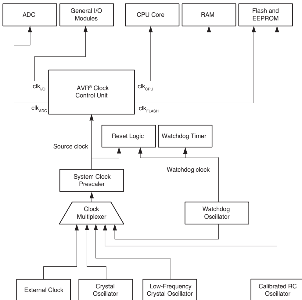
Figure 6-1. Clock Distribution
