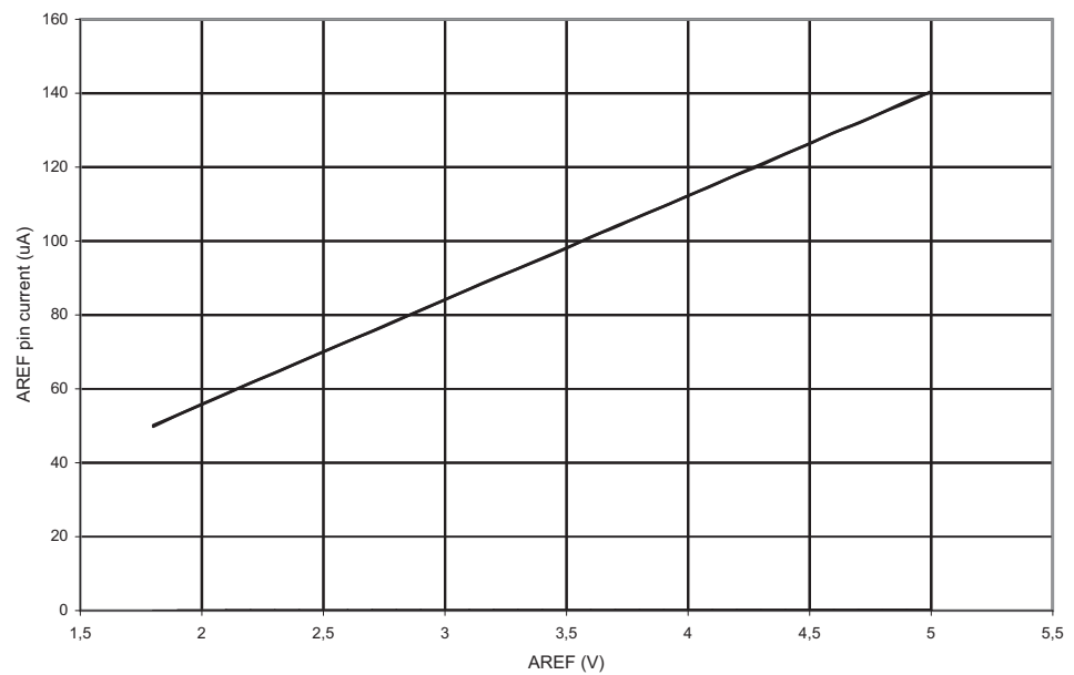
Figure 21-127. AREF Pin Current vs. Pin Voltage
