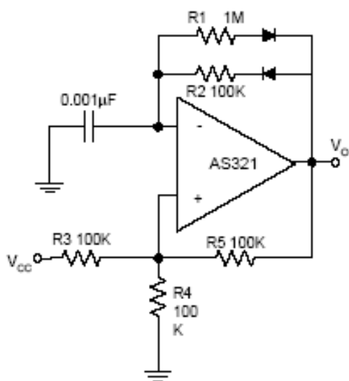
Pulse Generator
