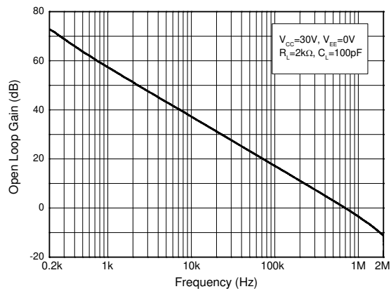
Open Loop Gain vs. Frequency
