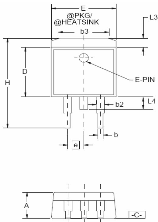
Figure 10. 3-Lead TO-252 Package
