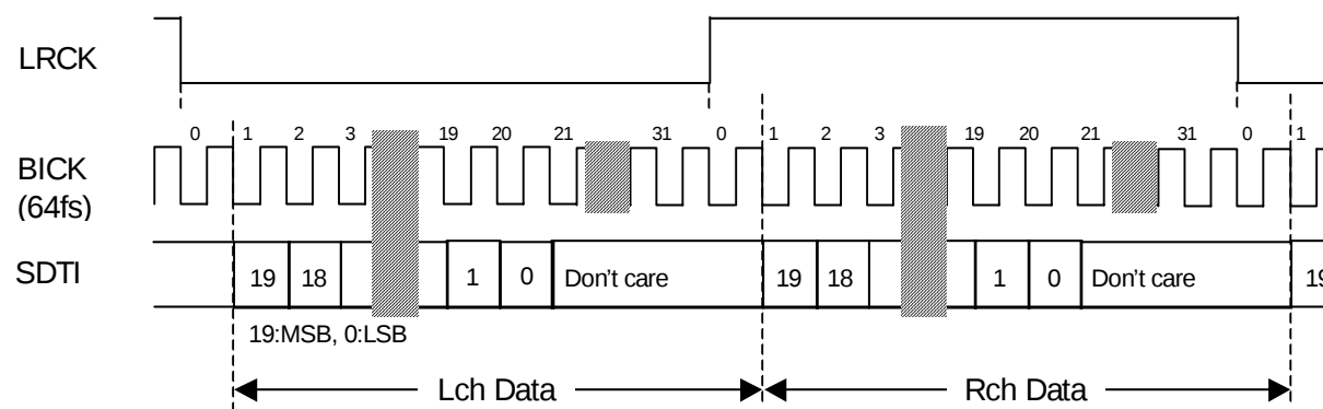
Figure 7. 20bit I 2 S Timing
