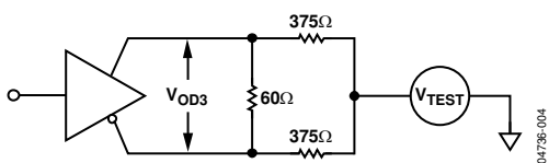
Figure 4. Driver Voltage Measurement
