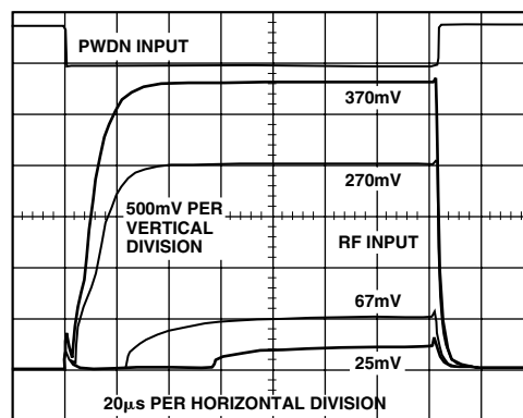
Figure 24. Output Response Using Power-Down Mode for Various RF Input Levels, Supply 3 V, Frequency 900 MHz, 0.01 \mu F Filter Capacitor
