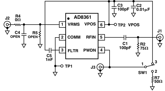
Figure 46. Evaluation Board Schematic, SOT-23-6L
