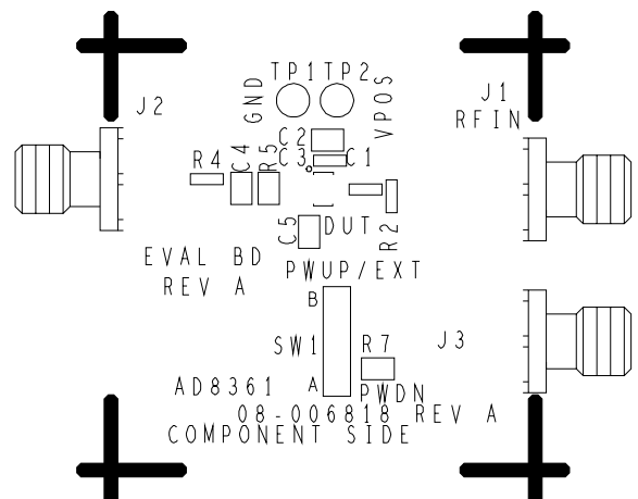
Figure 48. Silkscreen of the Component Side, SOT-23-6L
