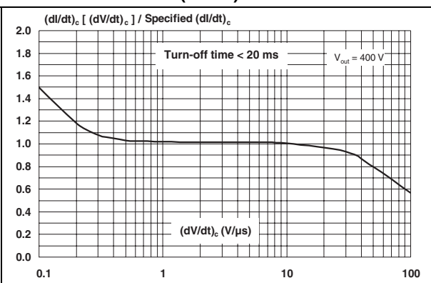
Figure 11. Relative variation of critical rate of decrease of main current (di/dt)_c versus (dV/dt)_c
