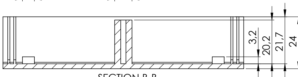
SECTION B-B
