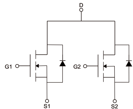
Schematic Diagram
