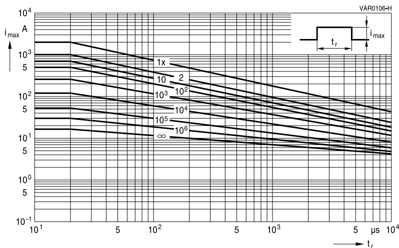
SIOV-S20K11 ... K40
