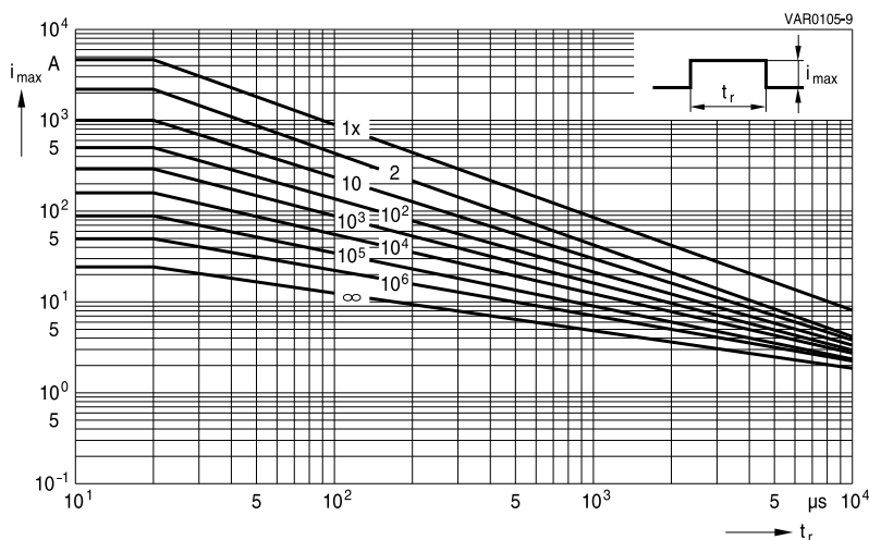
SIOV-S14K385 ... K1000
