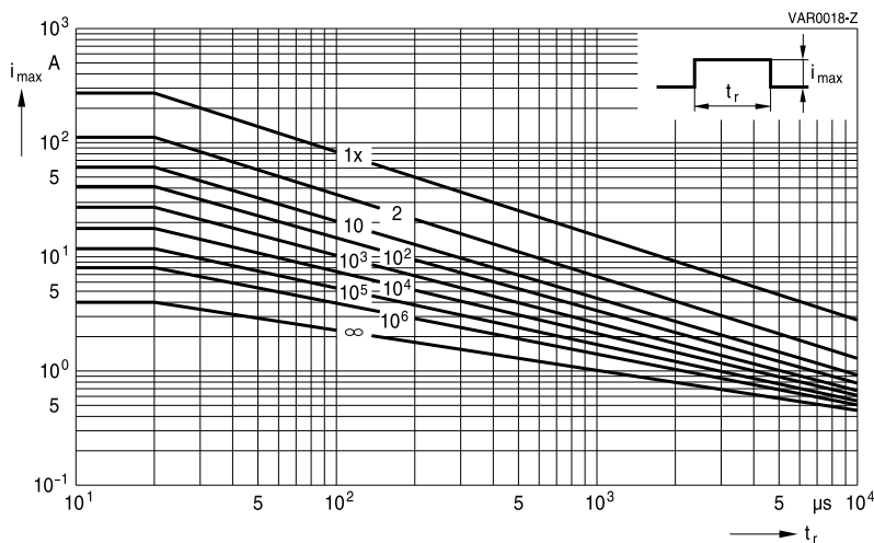
SIOV-S07K11 ... K40
