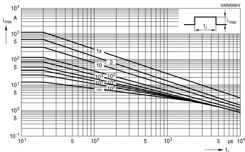
SIOV-S07K50 ... K460
