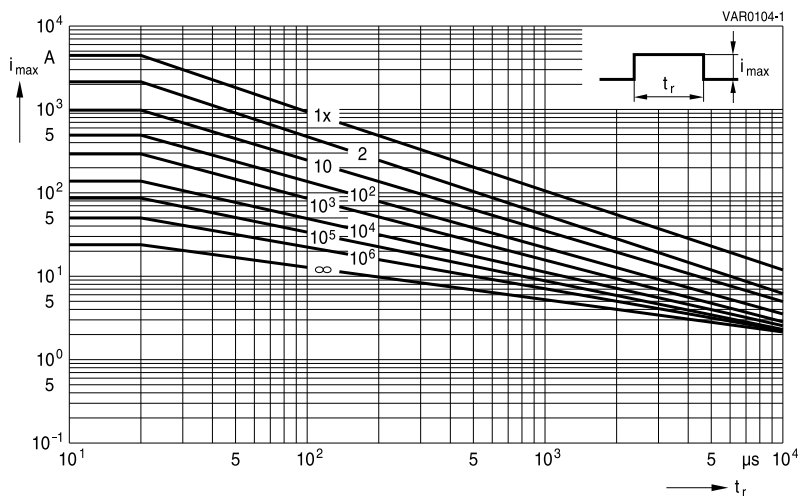
SIOV-S14K50 ... K320
