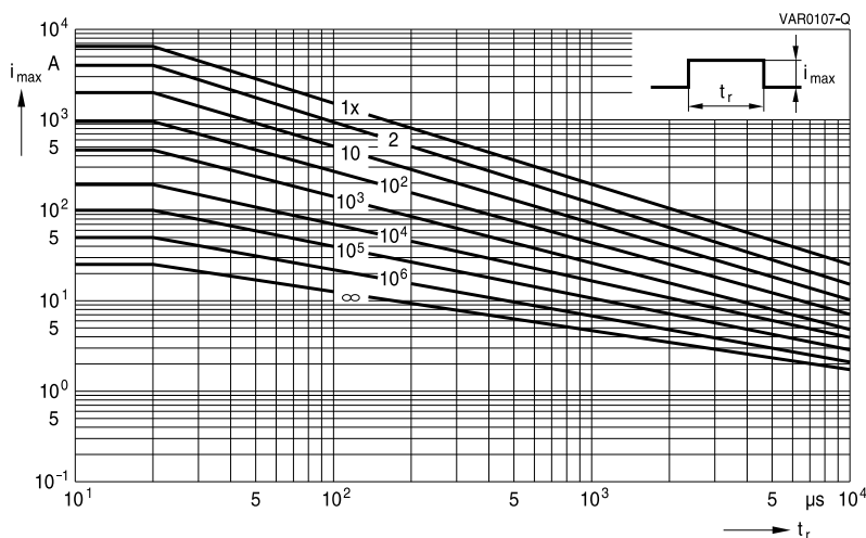
SIOV-S20K50 ... K115
