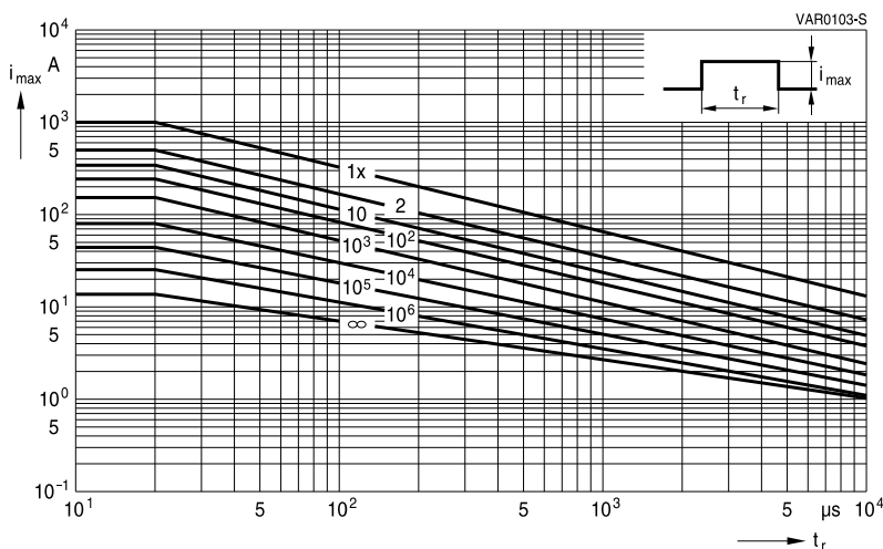
SIOV-S14K11 ... K40
