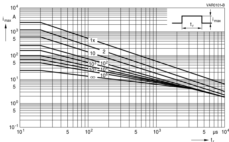
SIOV-S10K50 ... K320
