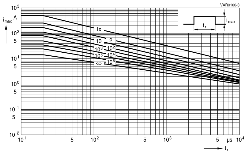
SIOV-S10K11 ... K40
