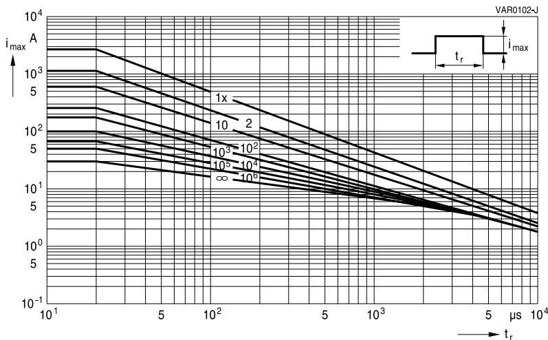
SIOV-S10K385 ... K680
