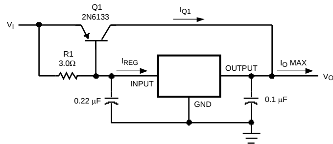
Figure 18. High Current Voltage Regulator
