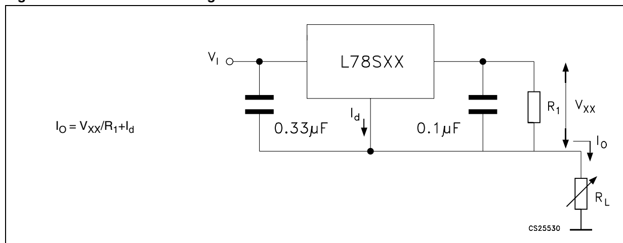
Figure 18. Constant current regulator
