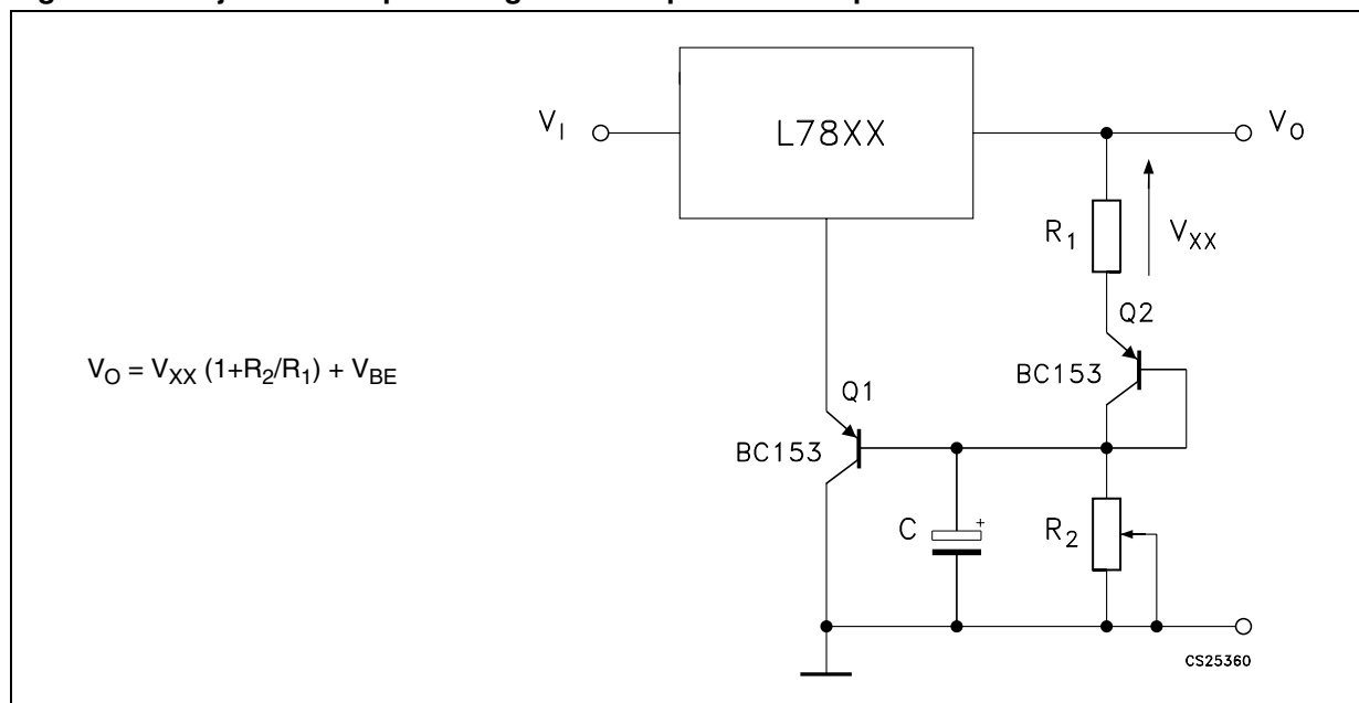
Figure 30. Adjustable output voltage with temperature compensation
