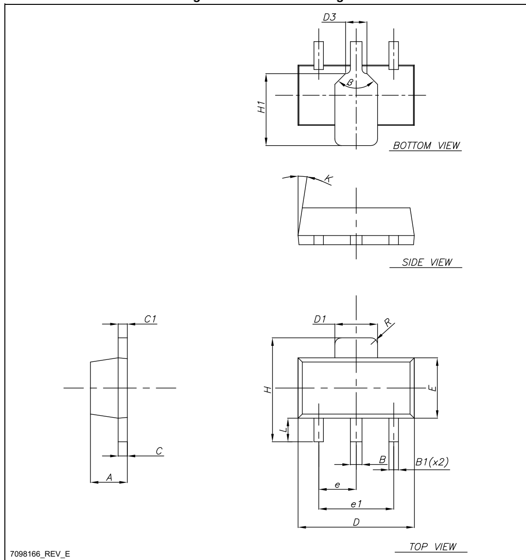
Figure 20. SOT-89 drawings
