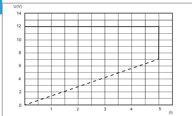
F FB78-1 Output voltage v output current (78.50)
