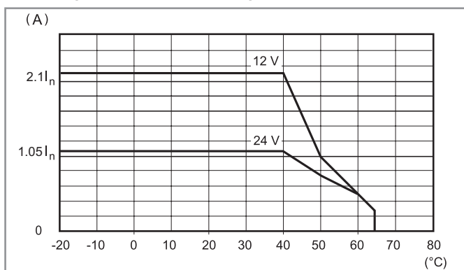
L78-2 Output current v ambient temperature (78.25)
