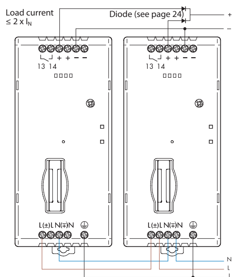
Wiring diagram for 78.1A
