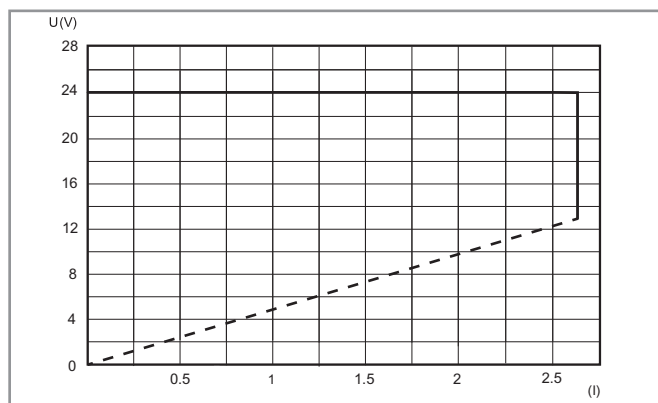
FB78-2 Output voltage v output current (78.60/61)
