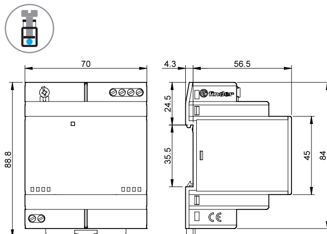
Type 78.1B Screw terminal
