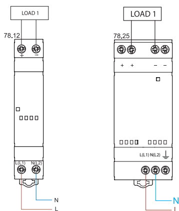
Dual polarity connection
