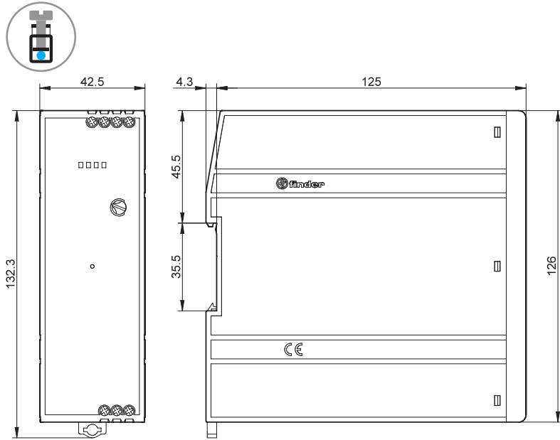
Type 78.2A Screw terminal
