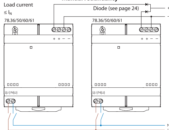
Manual redundancy
